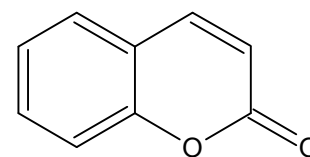
Kumaryna
