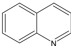
Chinolina
